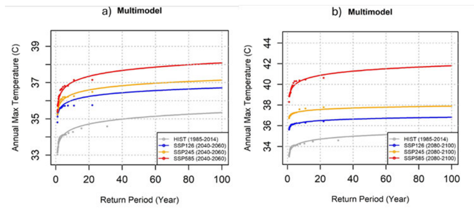
Figure 4-4 Comparison of Funafuti annual maximum daily temperature distributions for return periods of 1-100 years for historical (HIST: 1985-2014) and future (2040-2060 (a) and 2080-2100 (b)) timeframes, for low (SSP1-2.6), medium (SSP2-4.5) and very high (SSP5-8.5) emissions pathways. Results are based on the average of 5 CMIP6 climate models.
