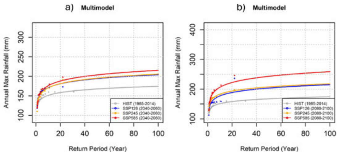
Figure 6-4 Comparison of Funafuti annual maximum daily rainfall distributions for return periods of 1-100 years for historical (HIST: 1985-2014) and future (2040-2060 (a) and 2080-2100 (b)) timeframes, for low (SSP1-2.6), medium (SSP2-4.5) and very high (SSP5-8.5) emissions pathways. Five CMIP6 models were assessed. Source [4].
