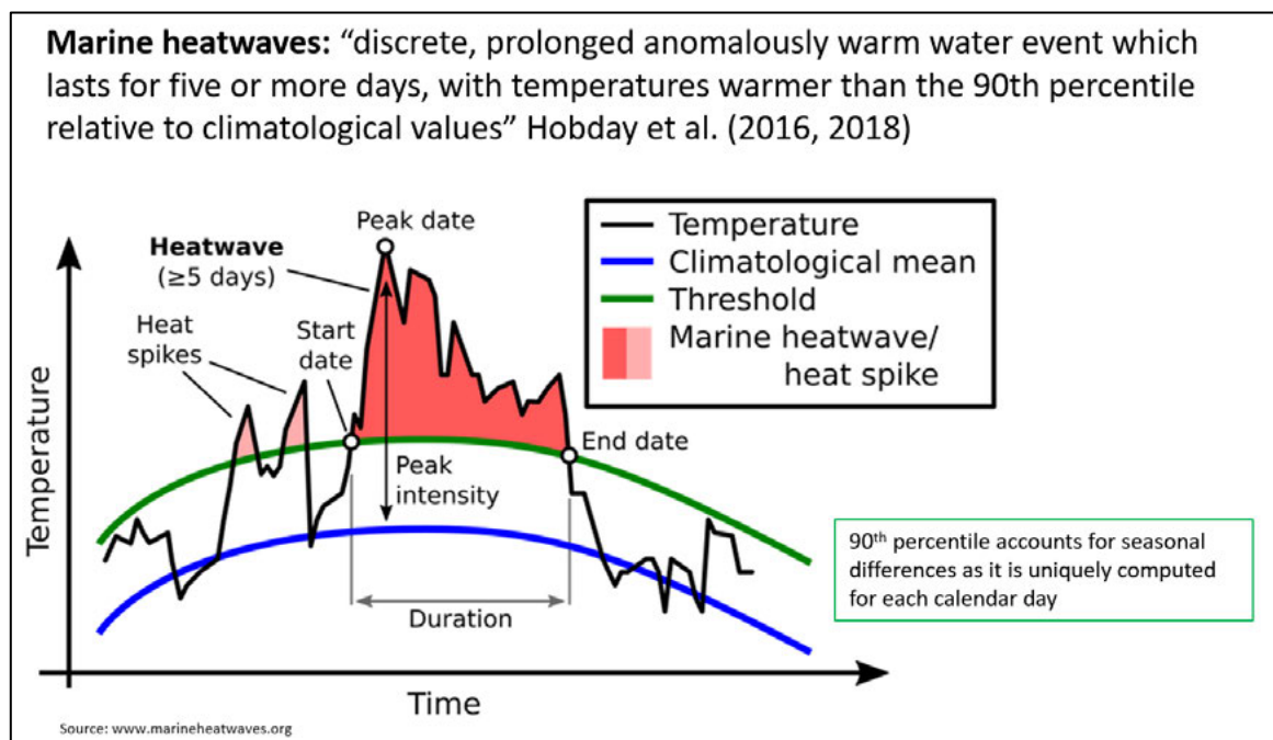
Figure 10-4 Diagram illustrating MHW definition: SST (°C) timeseries (black line) overlaid on the average SST (blue line) and the 90th percentile threshold (green line). When the SST exceeds the threshold for more than five days, it is defined as a MHW (red shading) [3, 4]. Heat spikes (pink shading) are not classified as a MHW because they are shorter than five days and are separated from the MHW by more than two days.
