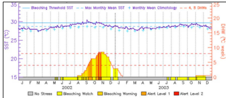
Figure 10-10 DHWs are plotted for a sample site in the Pacific along the bottom of the graph, corresponding to the accumulated threshold exceedance of SST above MMM. The 4-DHW and 8-DHW thresholds are shown as dashed, horizontal red lines. The colours that fill below the DHW line correspond to established satellite bleaching alert levels (see Table 10-2).
