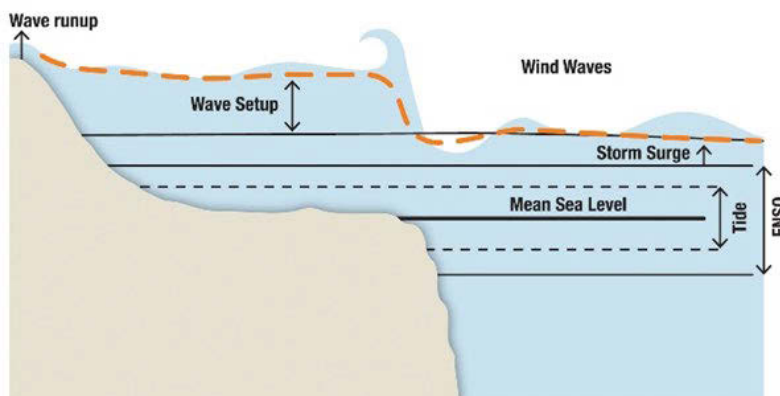
Figure 9-4 Schematic diagram of the contributions of extreme sea levels at the coast for a reef fronted island. The different contributions are tides, storm surge, storm waves and interannual sea level variability. Extreme sea levels are rare and may not always occur due to a tropical cyclone; for instance, if a storm surge happens at low tide, the total water level may not be extreme at the adjacent coastline.
